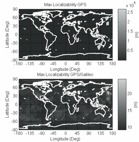
Figure 8. Maximum localizability for GPS (top) and combined GPS/Galileo (bottom)
