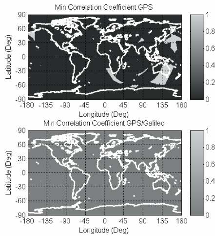
Figure 5. Minimum correlation coefficient ( \rho ) for GPS (top) and combined GPS/Galileo (bottom)
