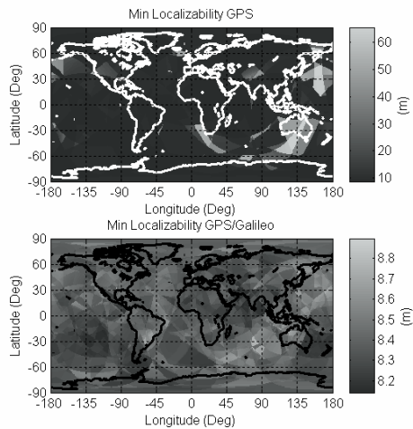
Figure 7. Minimum localizability for GPS (top) and combined GPS/Galileo (bottom)
