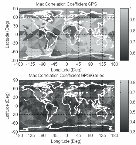
Figure 6. Maximum correlation coefficient ( \rho ) for GPS (top) and combined GPS/Galileo (bottom)
