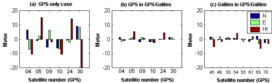
Figure 2. External Reliability for GPS and GPS/Galileo systems
