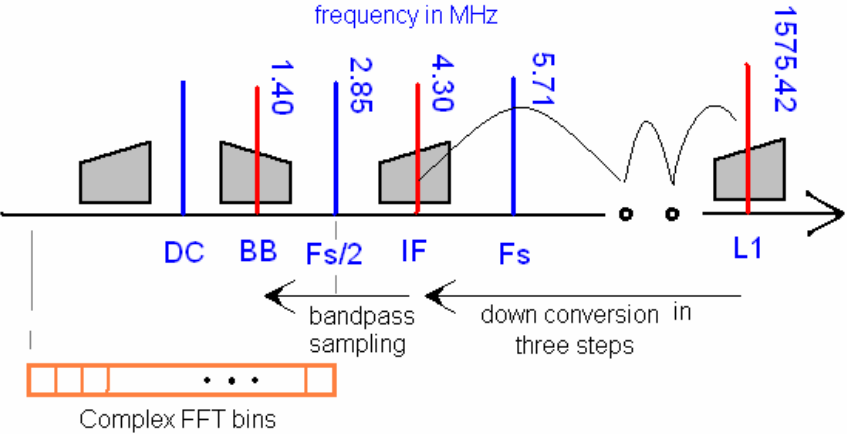
Figure 2. RF down-conversion and band-pass sampling diagram
