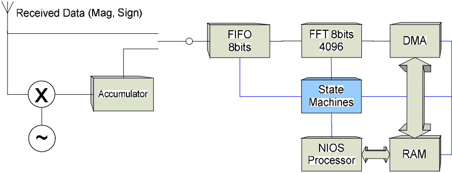
Figure 3. Simplified hardware block diagram
