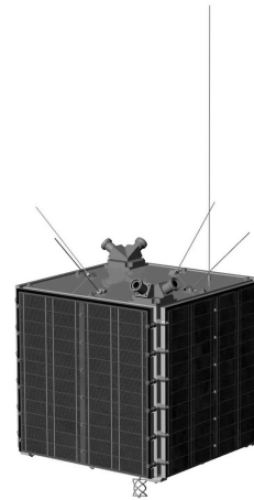
Figure 4. Drawing of the microsatellite ALMASat-I developed by the microsatellite laboratory, in the II School of Engineering, University of Bologna, Italy.
