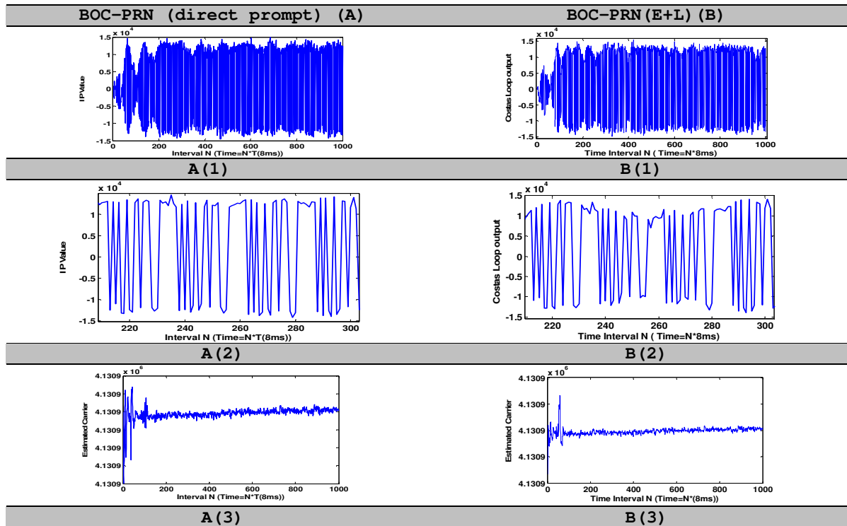
Figure 13 Real data tracking: plot of Pilot Channel Costas Loop output in time domain (updating intervals) (from SIGE Frontend(at 30March07,data1) Using BOC-PRN discriminators) A)BOC-PRN(Direct Prompt)discriminator; B)BOC-PRN(E+L)discriminator A/B(1)Costas Loop output (Navigation bit-secondary code in pilot channel);(2) zoom in on (1) between 220 and 300 integration intervals ;(3) Estimated carrier (around intermediate frequency of 4130400Hz).
