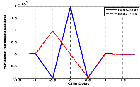
Figure 4 BOC-BOC ACF(Blue)&BOC-PRN CCF(red)
